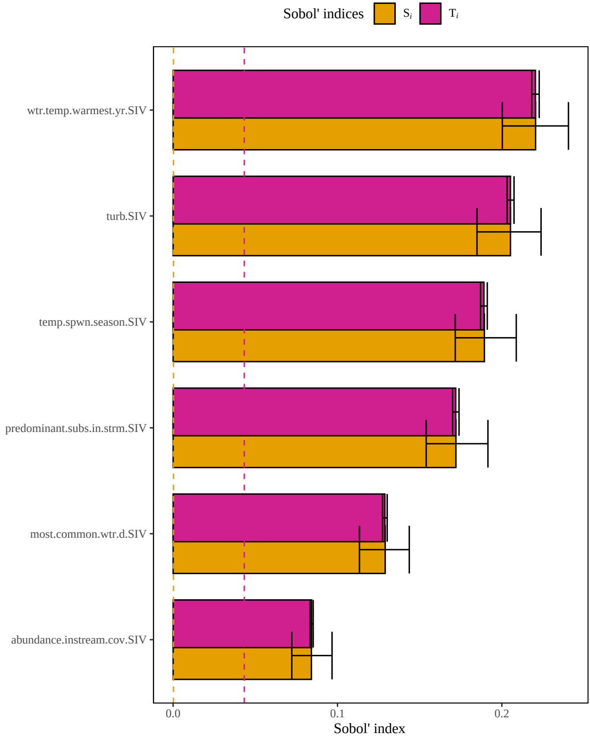
Figure 4. Results of a sensitivity analysis for the fallfishRivSpwn model based on an arithmetic mean structure. Dashed lines represent baseline numerical approximation error for S_i and T_i ( i.e. , dummy variables).
