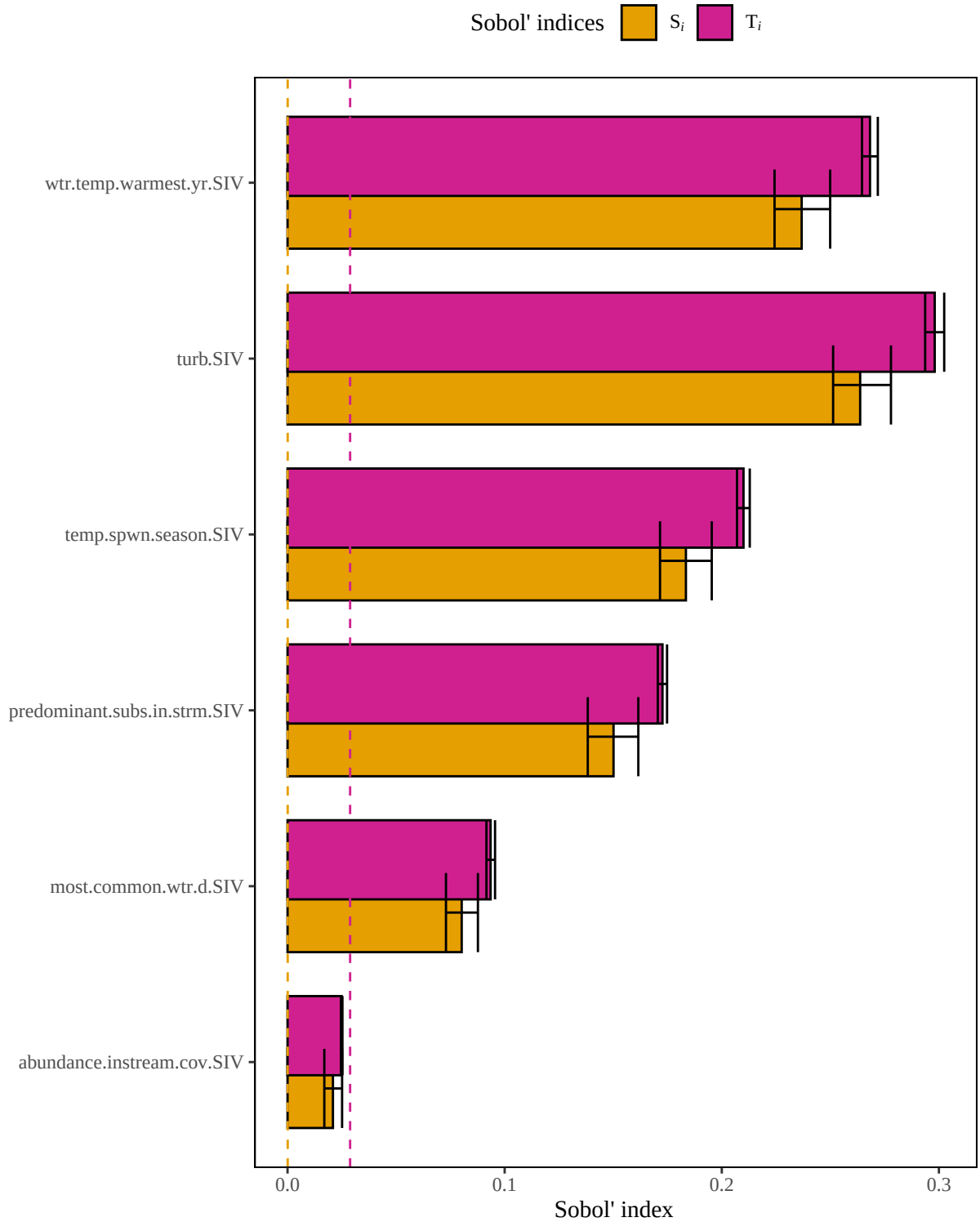
Figure 5. Results of a sensitivity analysis for the fallfishRivSpwn model based on a geometric mean structure. Dashed lines represent baseline numerical approximation error for S_i and T_i ( i.e. , dummy variables).
